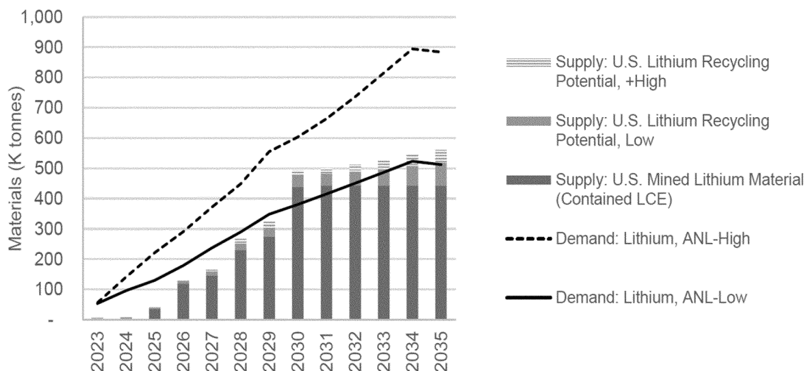
Figure 41: Potential U.S. Lithium Supply and Demand, ANL Study
