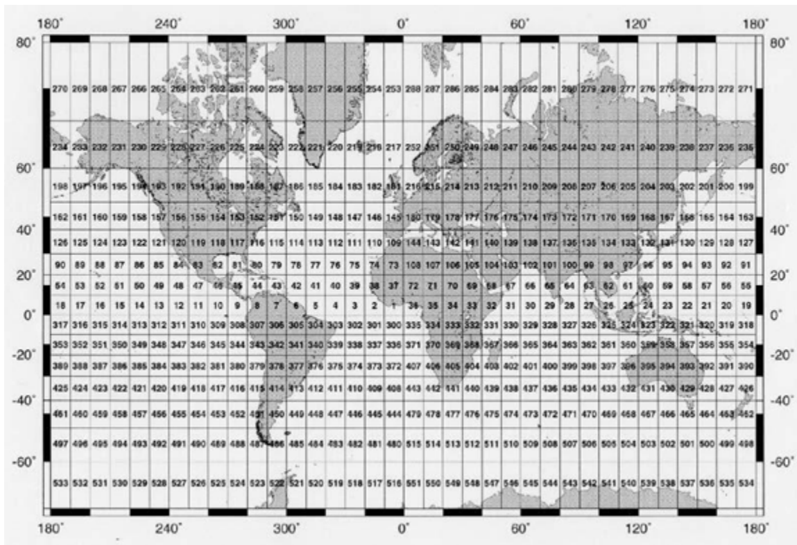
Figure F-5. Marsden Square Reference Diagram
