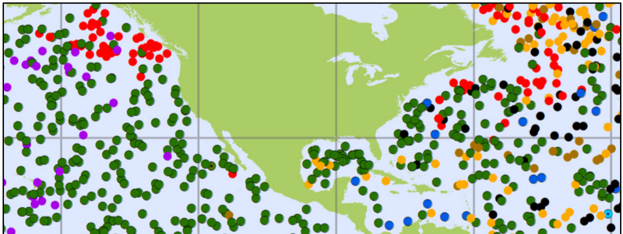
Figure 4-3. Service ARGO Float locations March, 2020 for Central and Eastern North Pacific, Central and Western North Atlantic, Gulf of Mexico, and Caribbean. Map from Service ARGO and GCOS/GOOS: WMO Joint Commission on Oceanography and Marine Meteorology (JCOMM). Colors indicate country of ownership: Green- USA, Red- Canada, Purple- Japan, Black- Germany, Orange- France, Brown- UK, Blue- EU.
