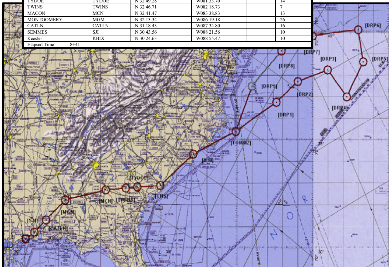
Figure E-1. Western Atlantic Flight Track WSRP-A61
