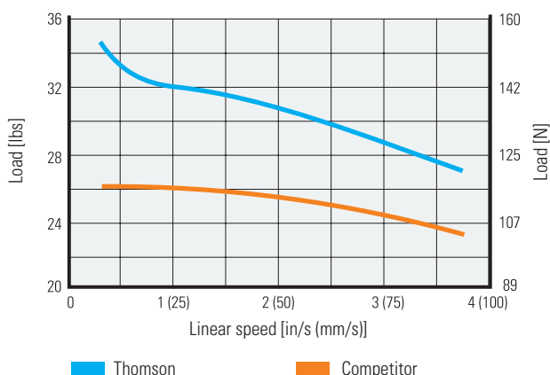
Load vs. Speed
